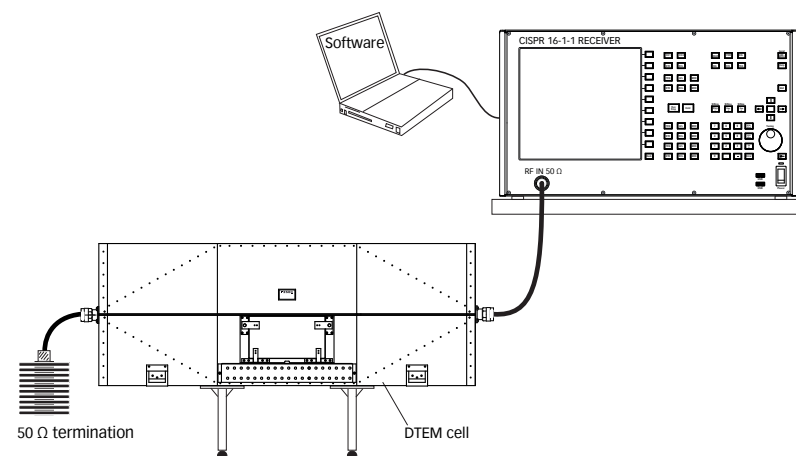
Example setup for emissions measurement
